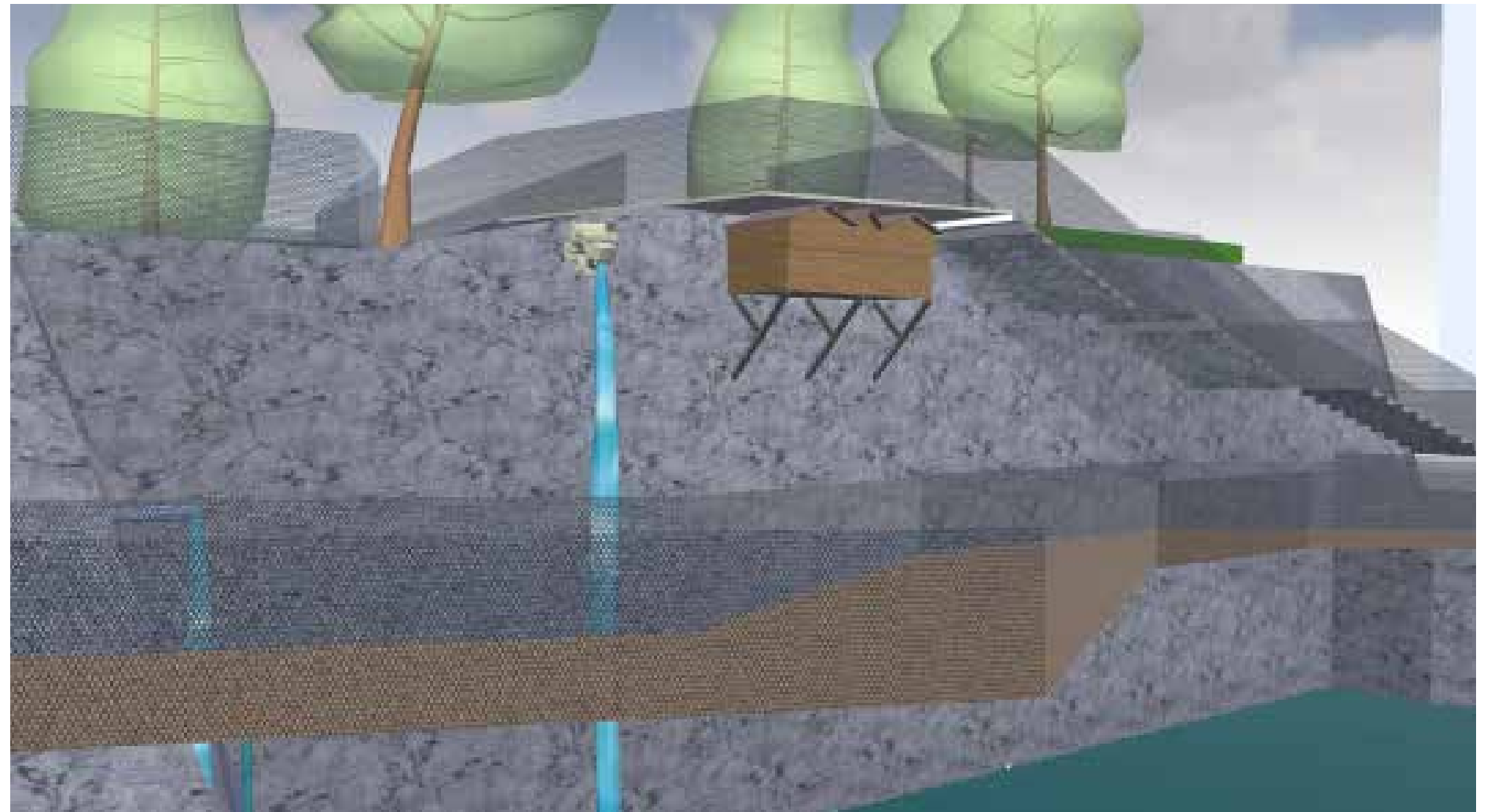
3D Concept model of quarry and reservoir
